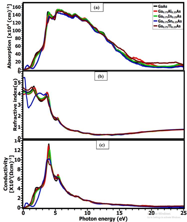
Fig. 10. Calculated absorption, refractive index and conductivity of GaAs and \text{Ga}_{0.75}\text{A}_{0.25}\text{As} ( \text{A}=\text{Al} , In, Sn and Tl) compounds.
