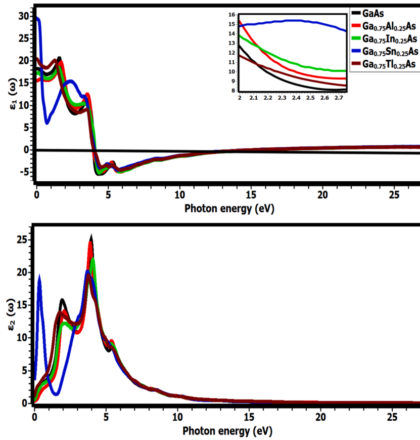
Fig. 9. Calculated real \epsilon_1(\omega) and imaginary \epsilon_2(\omega) of the dielectric function \epsilon(\omega) of GaAs and \text{Ga}_{0.75}\text{A}_{0.25}\text{As} ( \text{A}=\text{Al} , In, Sn and Tl) compounds.
