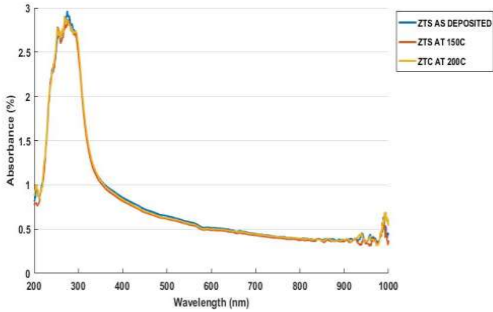
Figure 4: Graph of absorbance against wavelength for ZTS
