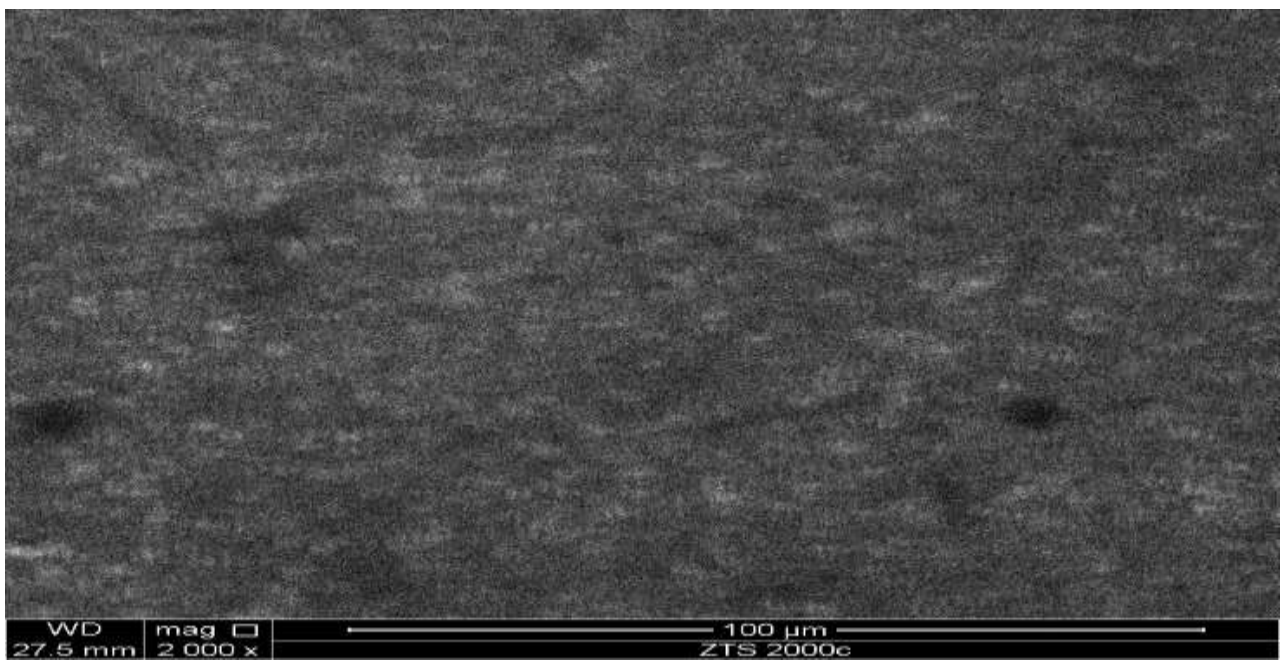
Figure 1c: SEM image of ZTS annealed at 200 °C
